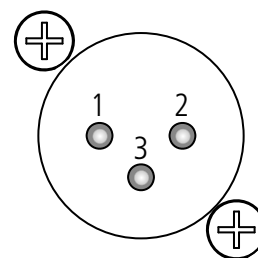
Male XLR connector
